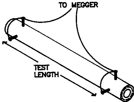
Figure 6-2 - Nail or “Pot Room” Test
